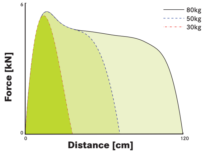
Fig. 1: Conventional via ferrata set: braking distances with 30 kg, 50 kg and 80 kg.
