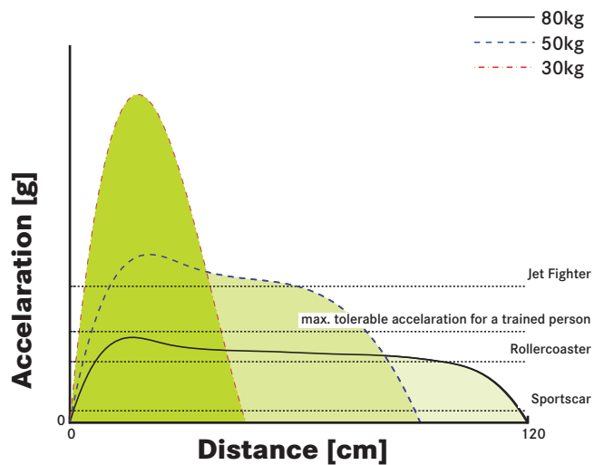
Fig. 2: Conventional Via Ferrata Set: Acceleration with 30 kg, 50 kg and 80 kg.
