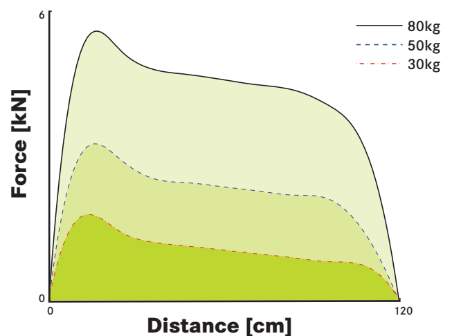
Fig. 3: EDELRID Cable Vario: braking distances with 30 kg, 50 kg and 80 kg.
